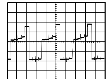
WF14 1DIV: 20V 20μsec Q 1522 Collector
