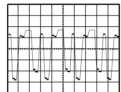
WF15 1DIV: 20V 20μsec Q 1512 Collector
